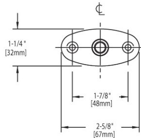
FLANGE DETAIL
